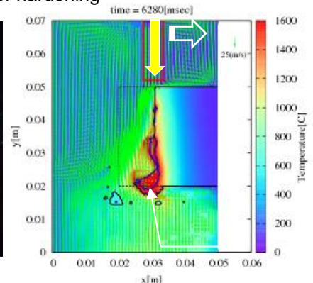
Fig.2 Laser cutting calculation (2D)
