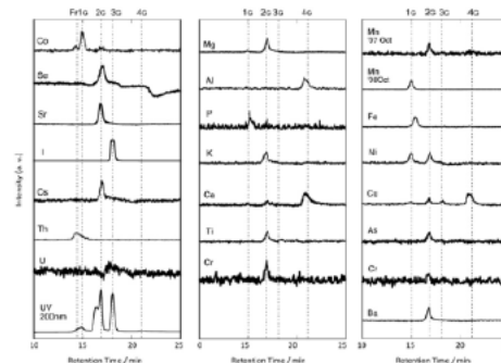
Fig. 5 - SEC-ICP-MS chromatograms obtained with the GL-W540 column and a 50 mM Tris-HCl buffer (pH 7.0). An SEC-UV chromatogram at 200 nm is also shown. The retention time of the SEC-ICP-MS chromatograms was adjusted to that of the SEC-UV chromatograms by subtracting a constant time lag between the UV-Vis detector and the ICP-MS.
