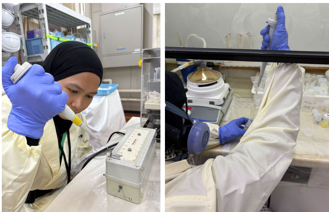
Sample analysis in ISCN
