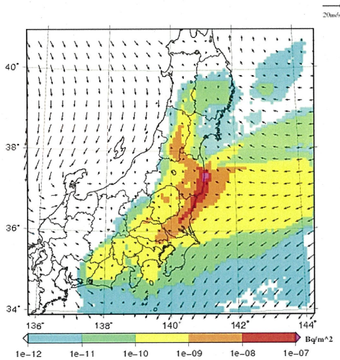
Surface deposition of I-131 at UTC= 2011-03-22_09h
