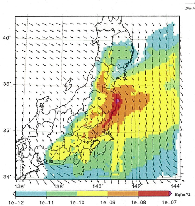
Surface deposition of I-131 at UTC= 2011-03-23_06h
