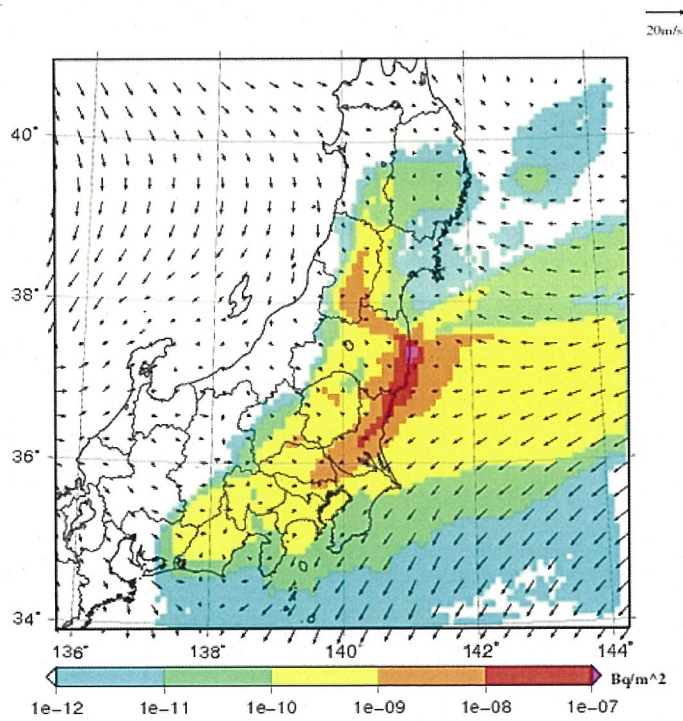
Surface deposition of I-131 at UTC= 2011-03-22_06h
