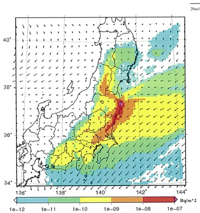
Surface deposition of I-131 at UTC= 2011-03-22_00h
