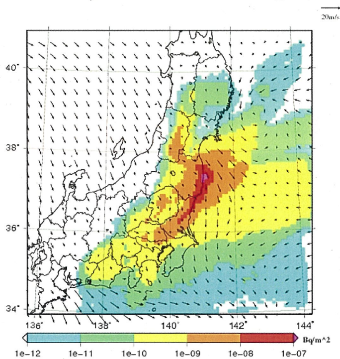
Surface deposition of I-131 at UTC= 2011-03-22_21h
