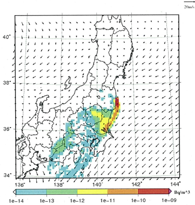
Surface concentration of I-131 at UTC= 2011-03-22_00h
