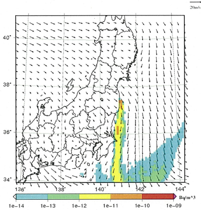
Surface concentration of I-131 at UTC= 2011-03-23_06h
