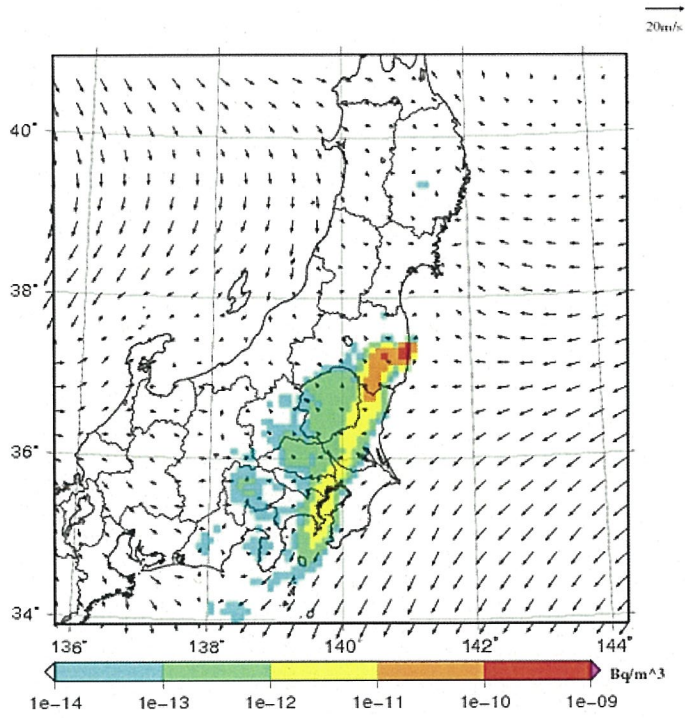
Surface concentration of I-131 at UTC= 2011-03-22_06h
