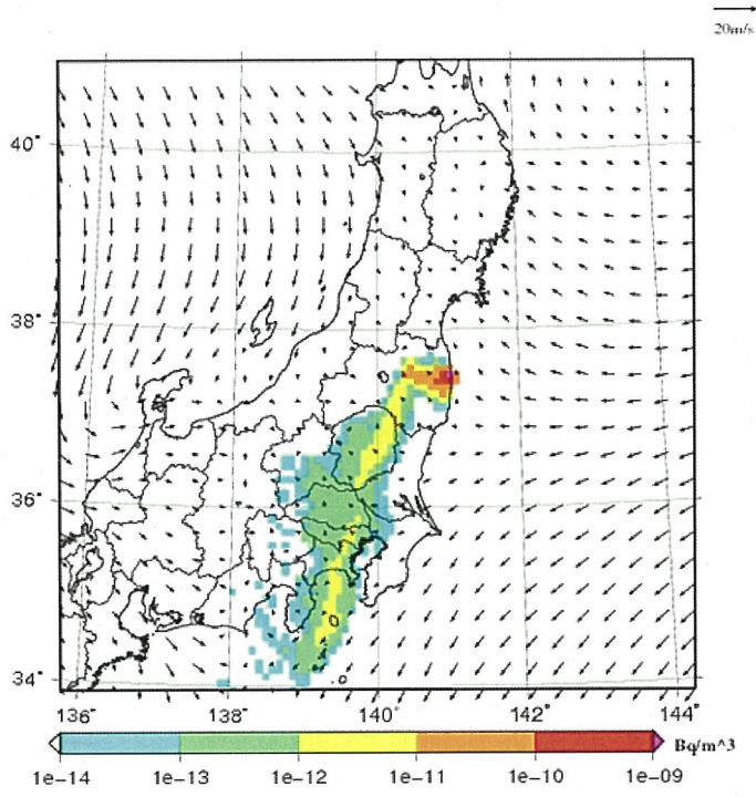
Surface concentration of I-131 at UTC= 2011-03-22_09h
