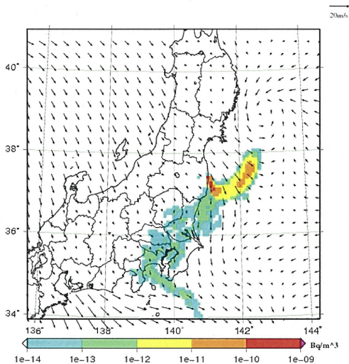
Surface concentration of I-131 at UTC= 2011-03-22_21h
